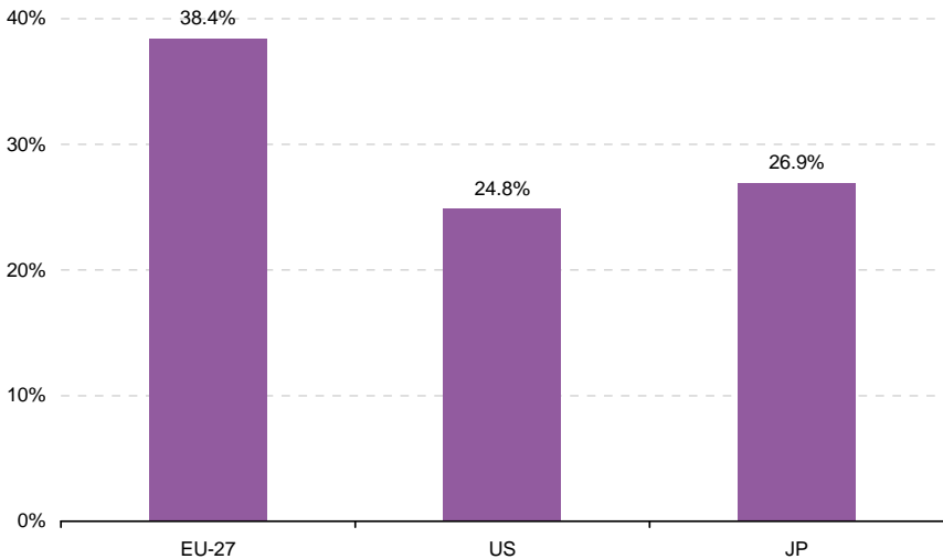
Graph 1: Overall tax-to-GDP ratio (incl. SSC) in the EU, US and Japan 2010, %
