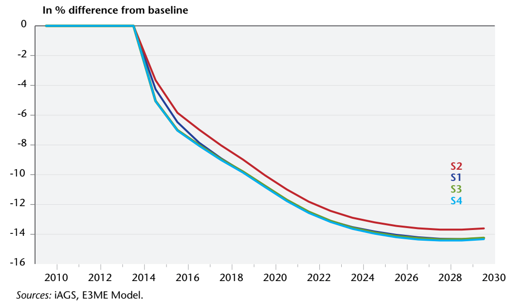
Figure 9. EU28 CO2 emissions by scenario,
