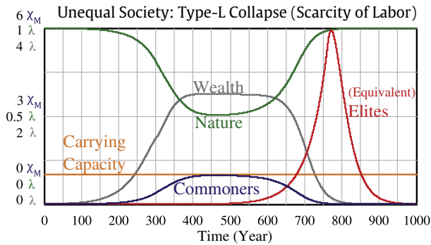
a) Population collapse following an apparent equilibrium due to a small initial Elite population when \kappa = 100 . This scenario also shows a different route to a collapse, in which, although Nature eventually recovers, population does not.
