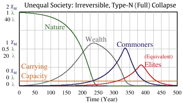
b) A fast full collapse due to both over-depletion and inequality ( \kappa = 100 ).
