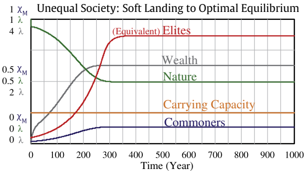
c) With moderate inequality ( \kappa = 10 ), it is possible to attain an optimal equilibrium by controlling the birth rates.
