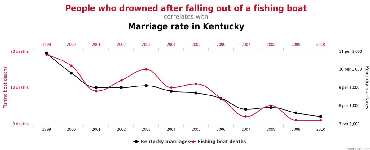
Figure 1: A correlation with r = 0.952407 [2].
